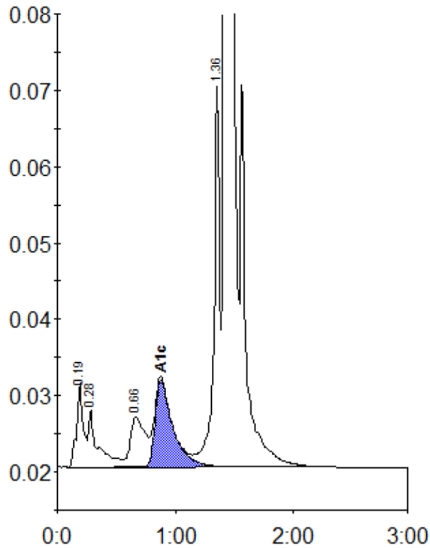
Peak table - ID: 10445388
